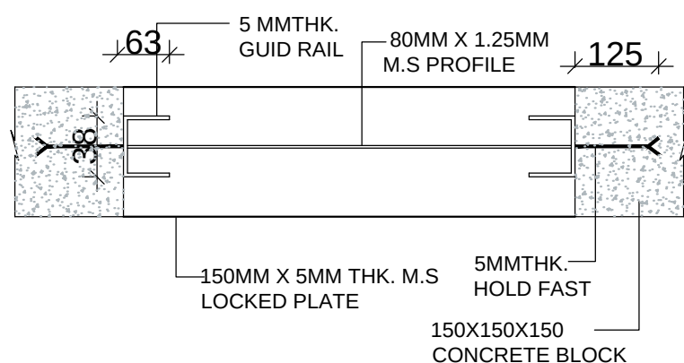
SECTION-CC
